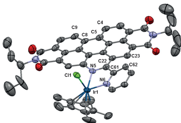
Figure 1. Molecular structure of [\text{Cp}^*\text{Ir}(\text{ab-PBI})\text{Cl}]\text{PF}_6 \mathbf{2} in the solid state (ellipsoids set at 50% probability; hydrogen atoms and counterion omitted for clarity).
